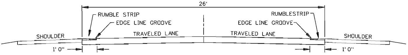
SECTION VIEW OF ROADWAY
